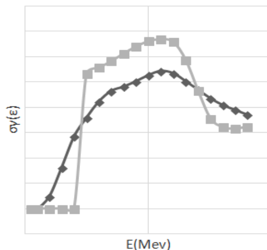
Fig.2 Cross section \Sigma\Gamma(E) of \gamma -emission \blacklozenge - p+^{14}_7N \rightarrow \gamma + \dots , \blacksquare - p+^{16}_8O \rightarrow \gamma + \dots
