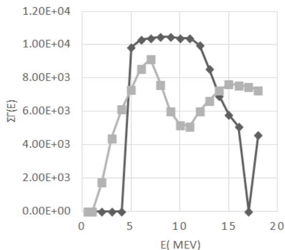
Fig.1 Cross section \Sigma\Gamma(E) of \gamma -emission \blacklozenge - p+^{12}_6C \rightarrow \gamma + \dots , \blacksquare - p+^{13}_6C \rightarrow \gamma + \dots
