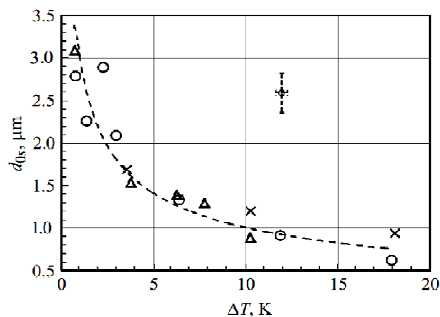
Fig. 4. Temperature dependence of the equilibrium thickness of the ELC layer of n -hexadecane on a metal according to measurement data: X – impurity dichroism, O – anisotropy of the induced birefringence, \Delta – viscosimetry [24, 27, 29]. The dotted line is the approximating trend.
