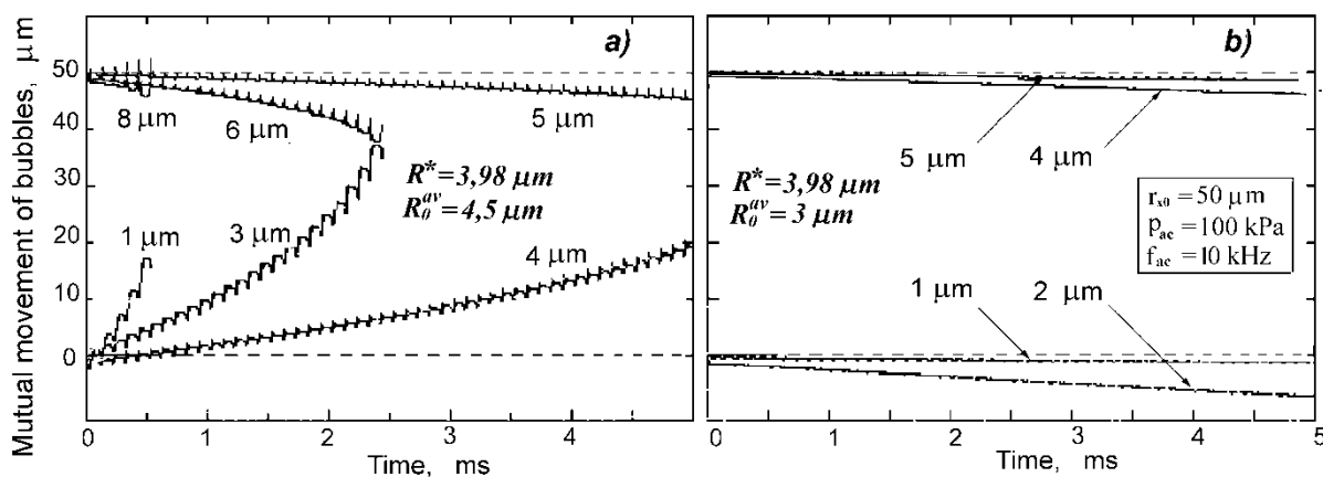
Fig. 5. Movement of the centers of two bubbles, pulsating in an acoustic field, with different values of their radii R_{l0} and R_{20} . The calculation was carried out under the same conditions and for the same five pairs of bubbles, which are shown in Fig.4. Pairs of bubbles with values R_0^{av}=4.5\text{ }\mu\text{m}>R^* (a) and R_0^{av}=3\text{ }\mu\text{m}<R^* (b) are shown.
