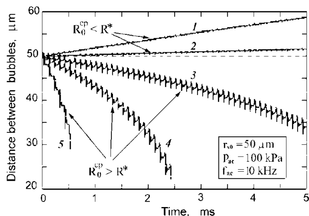
Fig.4. Change in the distance between two pulsating bubbles, with different values of their radii R_{I0} and R_{20} . The interaction of five pairs of bubbles with the following values R_{I0} and R_{20} : 1 – 4 and 2 \mu\text{m} ( R_0^{av} = 3 \mu\text{m} ); 2 – 5 and 1 \mu\text{m} ( R_0^{av} = 3 \mu\text{m} ); 3 – 5 and 4 \mu\text{m} ( R_0^{av} = 4.5 \mu\text{m} ); 4 – 6 and 3 \mu\text{m} ( R_0^{av} = 4.5 \mu\text{m} ); 5 – 8 and 1 \mu\text{m} ( R_0^{av} = 4.5 \mu\text{m} ); With the specified conditions of the US field the radius R^* = 3.98 \mu\text{m} .
