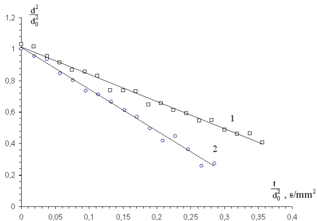
Fig.3. Squared diameters of burning droplets ( d_0 = 1.87 mm): ○ – Octadecane; ■ – Docosane.
